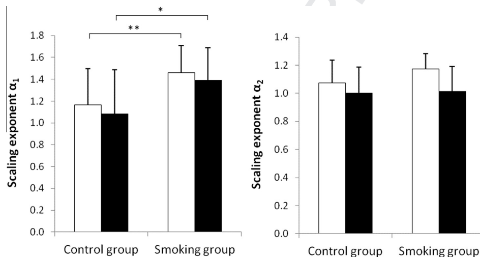
Fig. 1. Mean ± SD values of the scaling exponents \alpha_1 and \alpha_2 (as calculated in a DFA) during AS (empty bars) and QS (black bars) in the control and smoking groups. * P < 0.05; ** P < 0.01.
