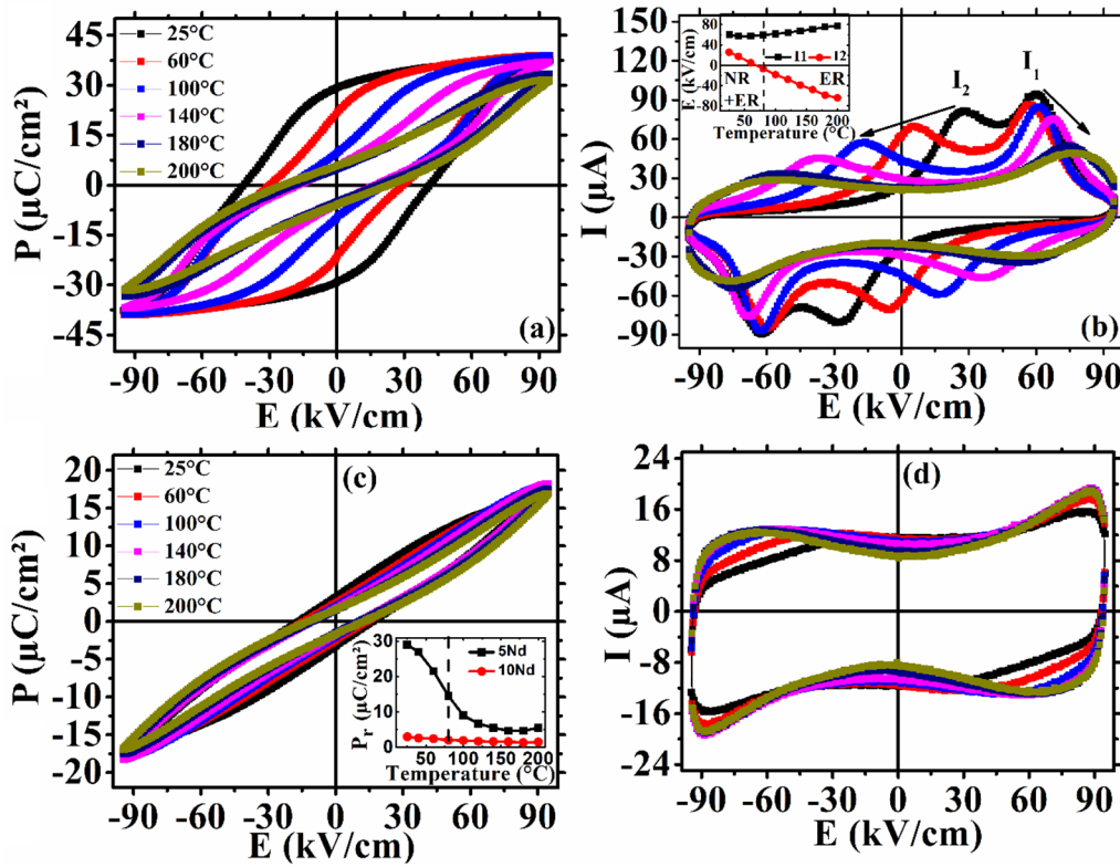
Fig. 9: Temperature-dependent (25 – 200°C) of the hysteresis loops for (a) 5NdNBT, and (c) 10NdNBT ceramics (Inset presents the temperature dependence of P_r for both samples). Temperature-dependent (25 – 200°C) of the I(E) curves for (b) 5NdNBT (Inset shows the temperature evolution of I_{1,2} peaks), and (d) 10NdNBT ceramics.
