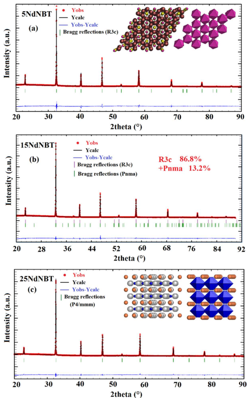
Fig. 3: Final Rietveld refinement plots of X-ray diffraction patterns for (a) 5NdNBT, (b) 15NdNBT, and (c) 25NdNBT: observed, calculated, and their difference. The calculated positions of Bragg reflections are marked by vertical markers. Insets show different structural views of the rhombohedral and tetragonal phases. For 5NdNBT, yellow spheres: Na/Bi/Nd cations, pink spheres: Ti cations, brown spheres: O anions, pink polyhedra: \text{TiO}_6 octahedra. For 25NdNBT, orange spheres: Na/Bi/Nd cations, blue spheres: Ti cations, grey spheres: O anions, blue polyhedra: \text{TiO}_6 octahedra.
