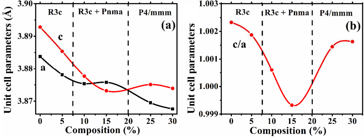
Fig. 2: (a) The variations of the equivalents lattice parameters and, (b) the c/a ratio in the studied compositions of the perovskite series x\text{NdNBT} , x = 0 - 30\% , as a function of \text{Nd}^{3+} amount.
