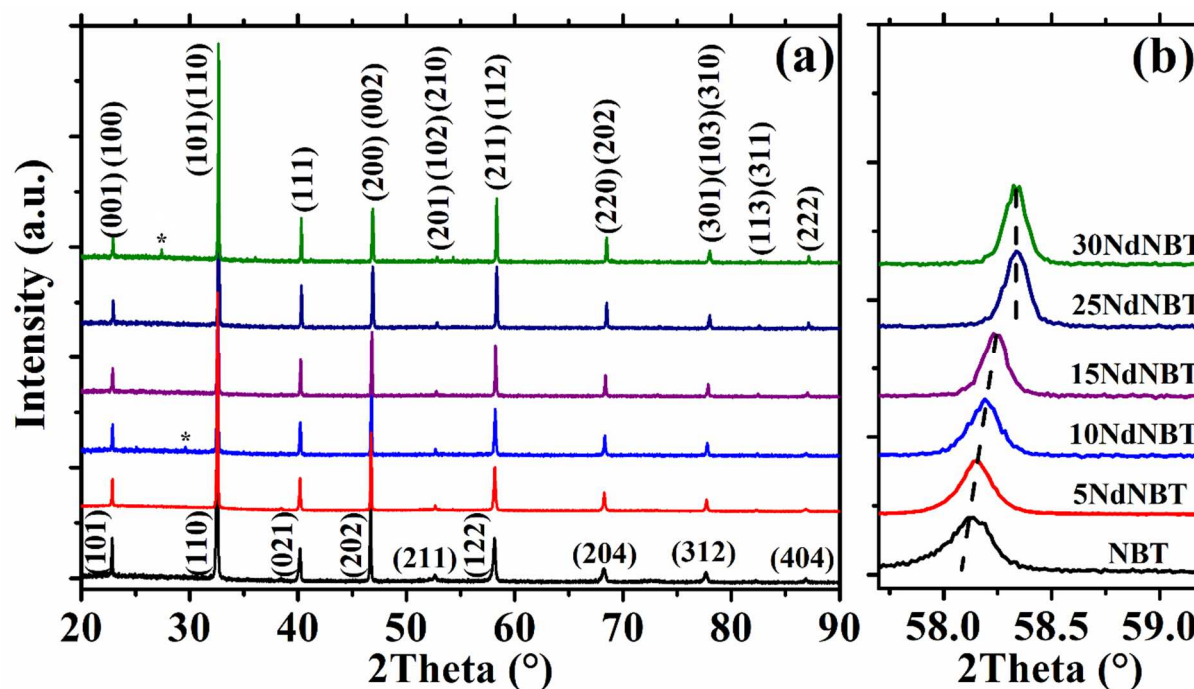
Fig. 1: Room temperature X-ray diffraction patterns of xNdNBT sintered ceramics: (a) x = 0 – 30%. (b): magnified (122) peak of the ceramics.
