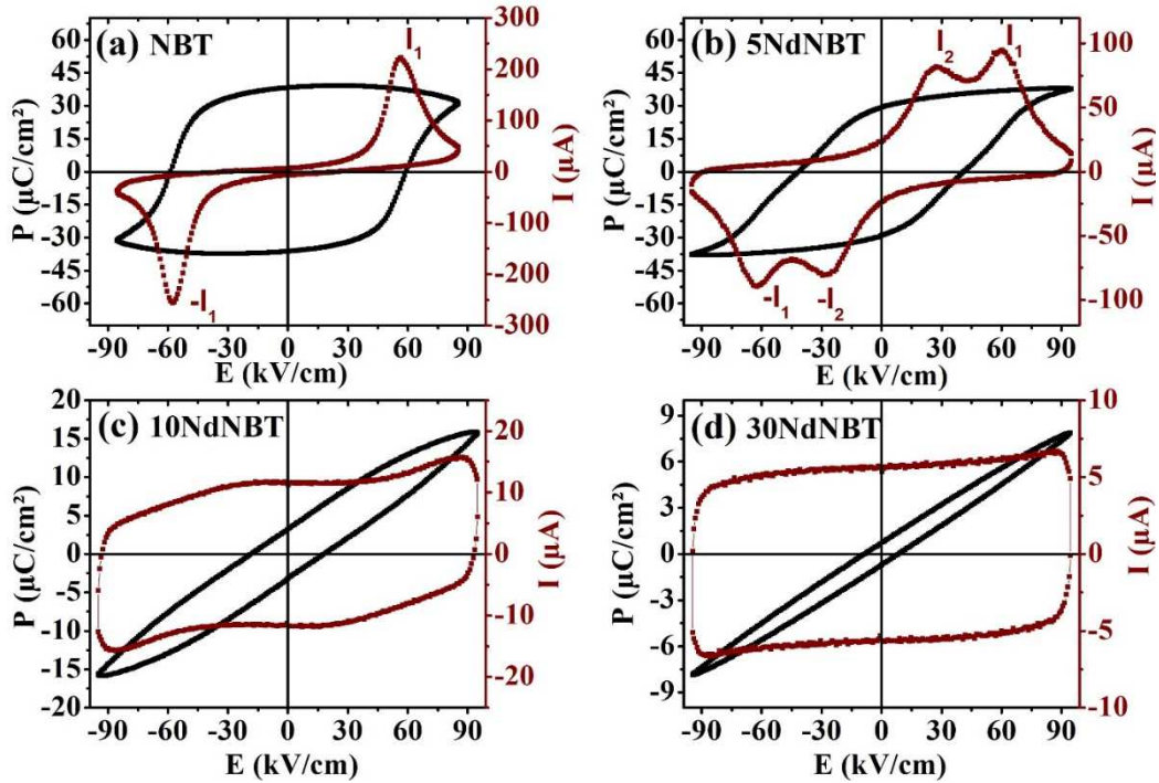
Fig. 8: Room temperature hysteresis loops, in addition to the current versus electric field curves for xNdNBT ceramics, with (a) x = 0 , (b) x = 5\% , (c) x = 10\% , (d) x = 30\% .
