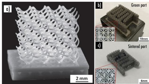
FIGURE 5. (a) Sintered alumina lattice structure [29]; (b) 3D printed octet structure obtained from a composite resin loaded with silver nanowire; (c) 3D printed octet structure after thermal post-processing [39].
