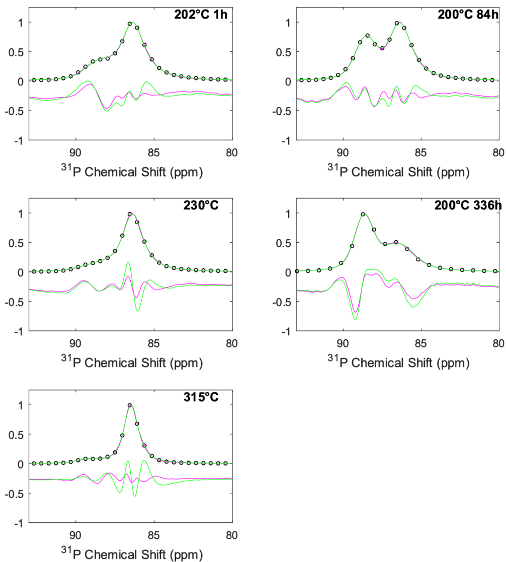
Figure S3: Fitted ^{31}\text{P} MAS NMR spectra of the 5 samples: 202-, 230-, 315- \text{Li}_3\text{PS}_4 and BM- \text{Li}_3\text{PS}_4 annealed at 200 °C for 84 hours and for 336 hours. The black circles stand for the experimental data, the magenta line shows the composite fit with 3 components; together with the difference plot below (scale x10). The corresponding data are shown in green for the 2-component fit.
