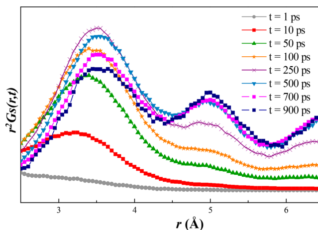
Figure 17. \text{Na}^+ -ion dynamics in \text{Na}_3\text{Sc}_{0.25}\text{Zr}_{1.75}(\text{SiO}_4)_{1.75}(\text{PO}_4)_{1.25} simulated at 773 K on different time scales. Vertical axis is the transformed self-part of the van Hove correlation function r^2 G_s(r, t) which is a measure of the probability of moving a distance r .
