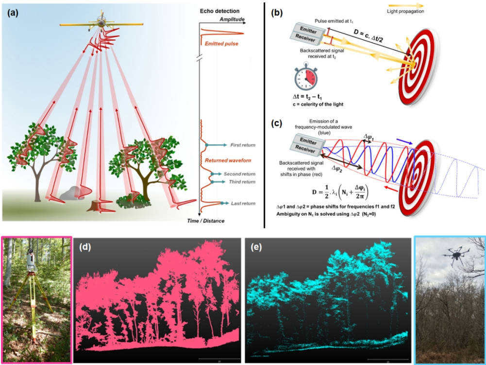
How light detection and ranging (LiDAR) works (a, b, c) and the mean to acquire LiDAR data from below or from above treetops (d, e). Upper-left panel (a): example of a non-stationary airborne LiDAR system (ALS) on board an aircraft. Upper-right panels (b, c): basic principles of time-of-flight vs. phase-shift LiDAR. Lower panels (d, e): data visualization of raw LiDAR point clouds extracted from both a stationary terrestrial LiDAR system (TLS) (Riegl VZ400) and a non-stationary ALS (YellowScan Vx20) covering the exact same study area in the Aigoual forest (France)
