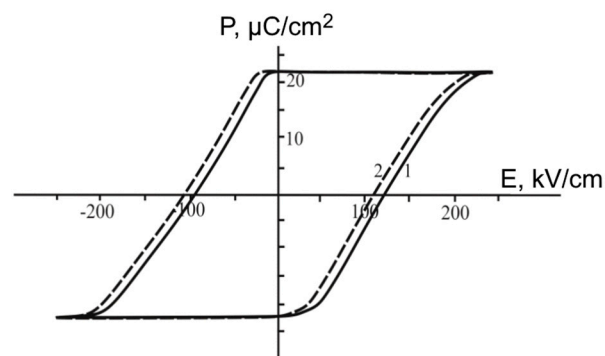
Figure 9. Dielectric hysteresis loop for BaZrO 3 /BaTiO 3 superlattice at the temperature of 20 °C: 1—without internal bias field, 2—with additionally applied field.
