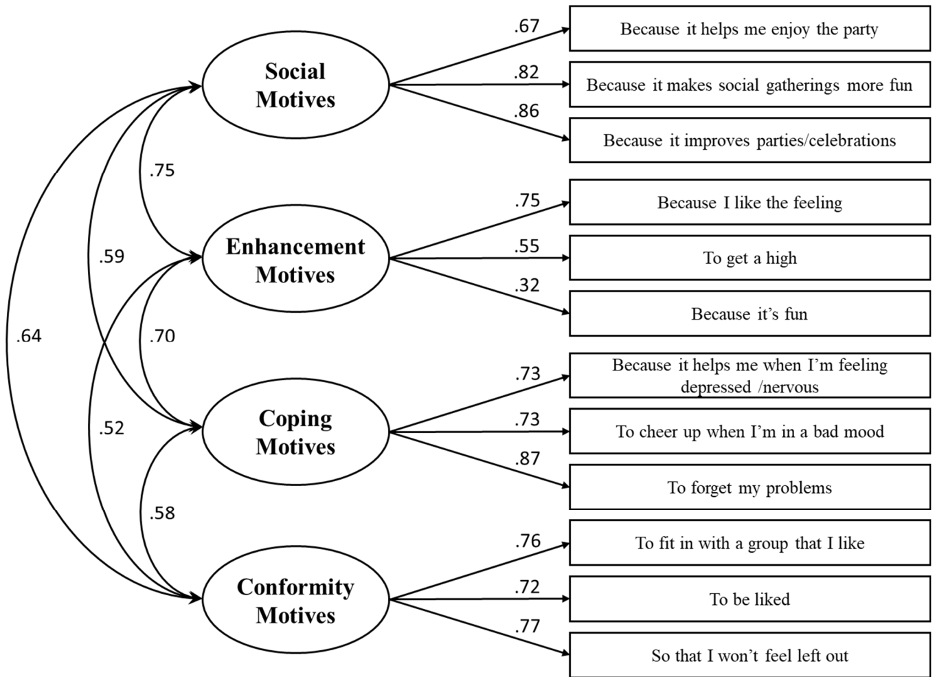
Figure 1. Confirmatory factor analysis model of the DMQ-R SF among patients with schizophrenia ( N = 113 ). All factor loadings (numbers above single-headed arrows) are significant at p < .001 except for Item “Because it’s fun” ( p = 0.01 ). All correlations (numbers above double-headed arrows) are significant at p < .002 .
