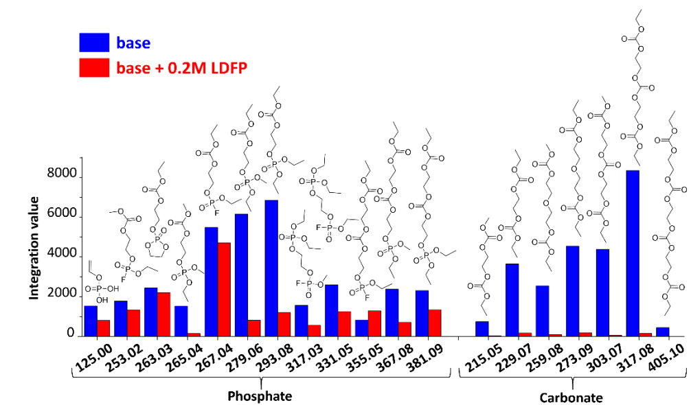
Figure 6. Phosphate and carbonate compounds analyzed by UHPLC-ESI-HRMS in electrolyte after 34 cycles (20 days) with base and base + 0.2M LDFP electrolytes. All peaks correspond to \text{Na}^+ adduct.
