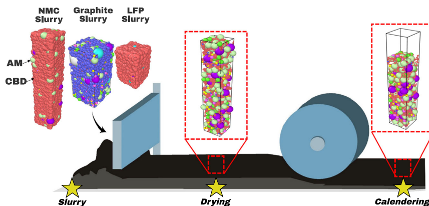
Fig. 1 Schematic of the first steps in the lithium-ion battery electrode manufacturing process which illustrates 3D-generated microstructures resulting from their mechanistic computational modeling. Our modeling methodology focuses first on the electrode slurry and can describe slurries made with different active material chemistries: \text{LiNi}_{0.33}\text{Mn}_{0.33}\text{Co}_{0.33}\text{O}_2 (NMC-111), Graphite, and \text{LiFePO}_4 (LFP).
