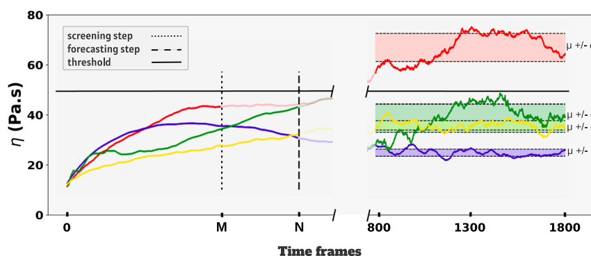
Fig. 4 Graphical representation of a few examples of mechanistic simulations with various slurry viscosity evolutions along with the time frames. We highlight the early numerical values to represent the viscosity curve taken into account in the screening, and forecasting steps if applicable, as well as the last 1000 numerical values serving for the calculation of associated simulation results. As it can be noticed, the numerical values in between are removed for the schematic representation of the framework's purpose. See Supplementary Figure 3 for the full-length simulations corresponding to these examples. M and N still represent the time frames selected to define time series for the screening and forecasting step. The threshold represents the upper limit for our range of interest.
