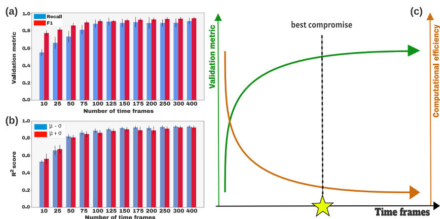
Fig. 5 Time frame selection based on the validation metrics from the training of different KNN models. a Evolution of the average Recall and F1_{score} as a function of the number of time frames. The latter defines the time series needed for the FPCA within the screening step of the framework. The black slight bar represents the standard deviation (SD) around the mean value of the validation metric. b Evolution of the average R^2_{score} as a function of the number of time frames for each KNN output. The latter defines the time series needed for the FPCA within the forecasting step of the framework. c Graphical representation of the best compromise between the validation metrics and the corresponding computational efficiency to calculate the simulation results for the time frame selection. The green trend illustrates the results from a and b and the orange one is a simplification of the evolution of the computational efficiency function of time frames to clarify the overall compromise. The expected best compromise is illustrated where both trends plateau.
