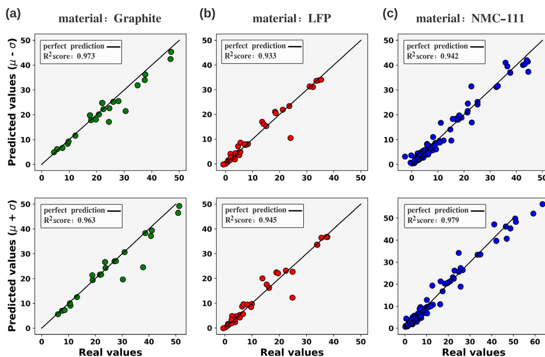
Fig. 6 Regression plots to evaluate the predictive capabilities of the KNN regression for the fitting of \mu \pm \sigma . a Comparison of the predicted values against the real values, for mechanistic simulations associated with the Graphite within the testing data set. b Comparison of the predicted values against the real values, for mechanistic simulations associated with the LFP within the testing data set. c Comparison of the predicted values against the real values, for mechanistic simulations associated with the NMC-111 within the testing data set.
