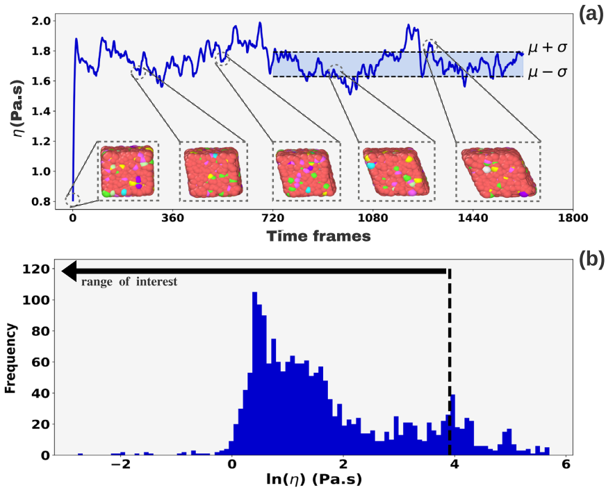
Fig. 2 Data treatment of the NEMD simulation for the assessment of the simulation results. a The slurry microstructure evolution and associated viscosity ( \eta ) during the NEMD simulation were handled to assess the slurry viscosity at a given shear rate ( \dot{\gamma} ). The last 1000 viscosity values from a single simulation are used as a vector to calculate an average value ( \mu ) and a standard deviation ( \sigma ). These latter values enable to color-code the slurry viscosity evolution within a box, where the two limits are the average plus and minus the standard deviation ( \mu \pm \sigma ). b Empirical natural log distribution of the average slurry viscosity value ( \eta ) associated with the mechanistic simulations carried out in this study. The black arrow illustrates the range of interest for the simulated viscosity values.
