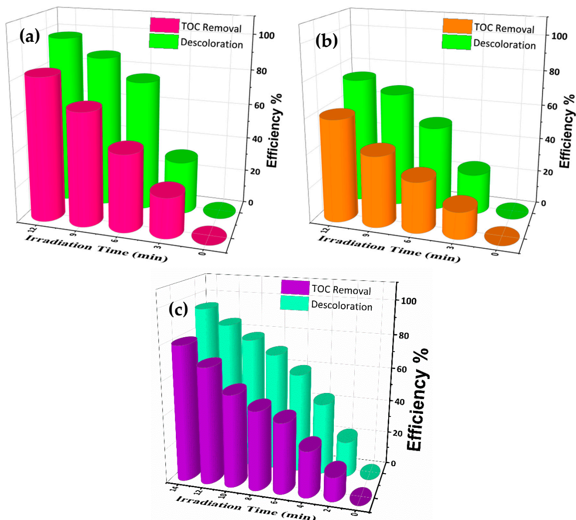
Figure 14. TOC removal and decoloration as a function of time of (a) Rhodamine B, (b) Orange G and (c) RhB-MB in the presence of the BiP-500 photocatalyst.
