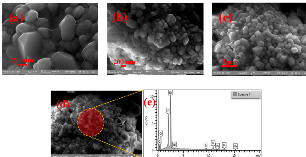
Figure 3. SEM images and EDX spectrum of BiPO 4 treated at 500 °C.
