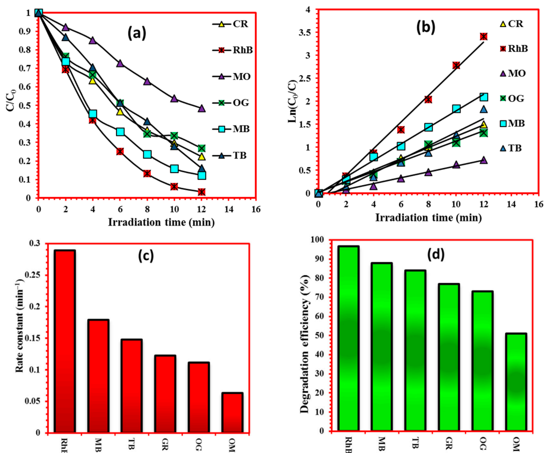
Figure 11. (a) Variation in C_t/C_0 ratio as a function of time for the different pollutants (RhB, MB, TB, CR, OG, OM); (b) pseudo-first-order kinetics of the photodegradation mechanism for all pollutants; (c) evolution of the associated apparent rate constant k_{obs} as a function of pollutants; (d) efficiency of degradation after irradiation time of 12 min for the degradation of different pollutants.
