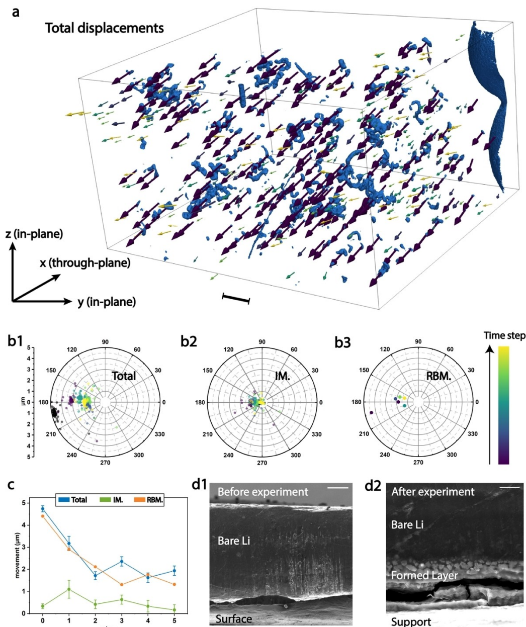
Figure 4. Dynamics study of the time-resolved volumes (a) The 3D rendering of tracked total displacements (rigid body movement RBM + intra-particle movement IM) for all the particles in time steps. The size of arrows indicates the magnitude of movement, and its color indicates the time step. And the time step color bar is shared between the (a) and (b) plots. The scale bar in (a) from left to right, b1-3) are respectively polar plots for total displacements, RBM, and IM projected on the plan XY (the movements on z direction are quasi-null), showing the distribution of motion vectors for each tracked particle at time t . The latitudes represent angle formed between the vector and the x axis at plan XY, and the longitude its module of the vector. c) plot of average module of displacement for all tracked particles with time. d1-2) SEM images comparison of the intersection of the pristine lithium foil and the post-experiment one. A thick non-uniform micrometric layer is formed on the surface of Li. The scalar bar in d1 represents 100 \mu\text{m} , and 20 \mu\text{m} for d2.
