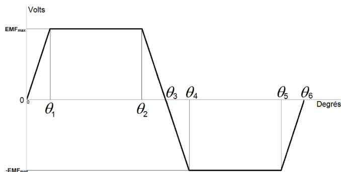
Figure 8 Curve of an EMF generated at 125 rpm
