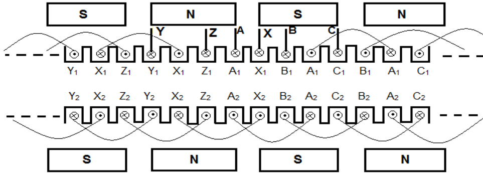
Figure 3 Axial flux PMSM electrical diagram
