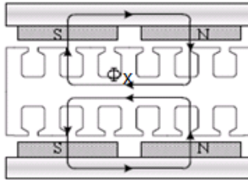
Figure 3 Axial flux PMSM electrical diagram
