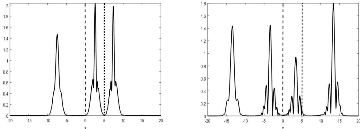
FIGURE 11. Numerical solution after the second defect interaction, t = 0.0873 (left) and t = 0.1371 (right).
