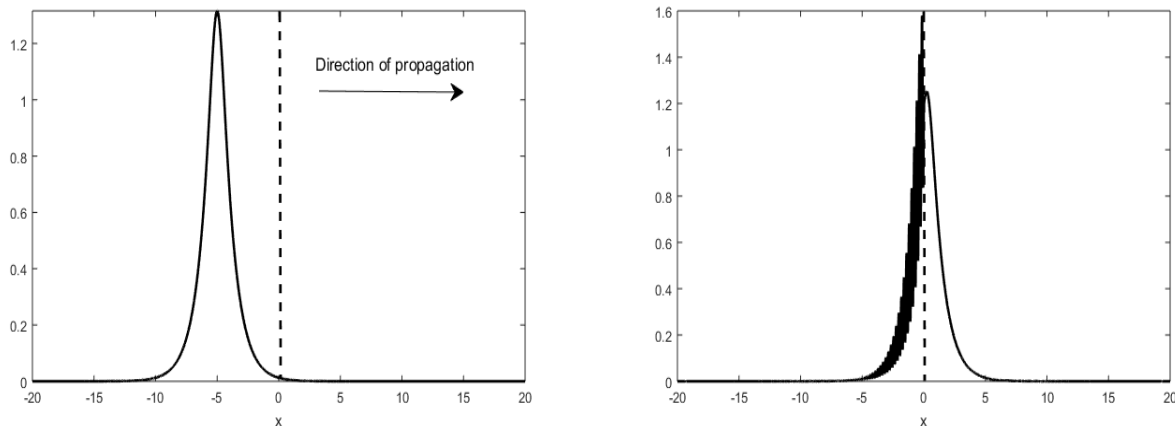
FIGURE 4. Initial profile and solution profile when interacting with the defect for Z = 10 at t = 0.174 .
