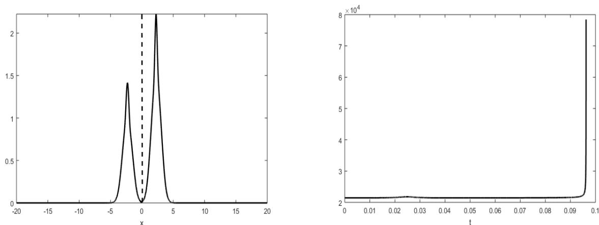
FIGURE 10. Numerical solution after the first defect interaction ( Z_1 = 80 and Z_2 = 0 ), t = 0.0442 (left) and plot of the norm \|(u_{\mathbf{t}}^{Z_1})_x\|_{L^2}^2 (right).
