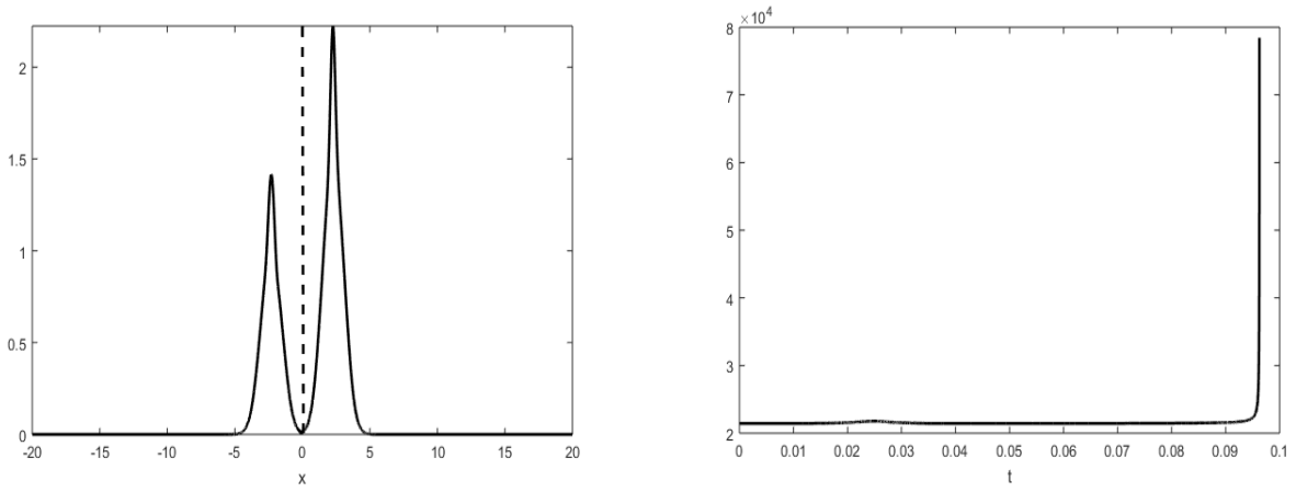
FIGURE 10. Numerical solution after the first defect interaction ( Z_1 = 80 and Z_2 = 0 ), t = 0.0442 (left) and plot of the norm \|(u_t^{Z_1})_x\|_{L^2}^2 (right).
