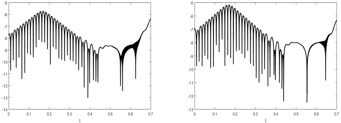
FIGURE 3. Plot of \log \frac{M^{n+1} - M^n}{M^n} (left) and \log \frac{E^{n+1} - E^n}{E^n} (right) versus time.
