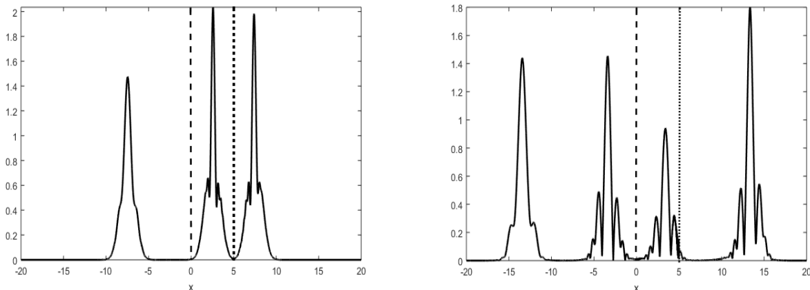
FIGURE 11. Numerical solution after the second defect interaction, t = 0.0873 (left) and t = 0.1371 (right).
