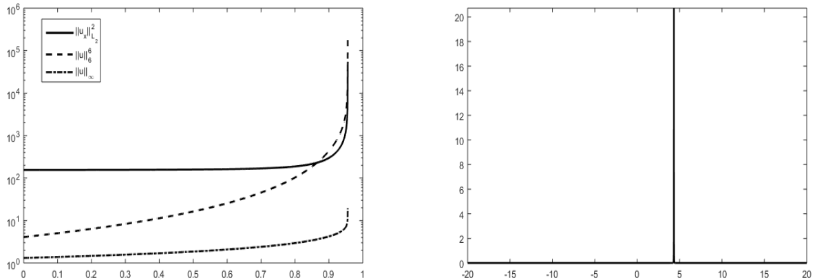
FIGURE 2. Discrete versions of \|u_x\|_{L^2}^2 , \|u\|_{L^6}^6 and \|u\|_{L^\infty} versus time (left) and spatial singularity formation at t = 0.9557 (right).
