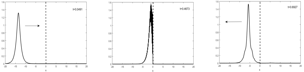
FIGURE 6. Solution profile for Z = -10000 at different times.
