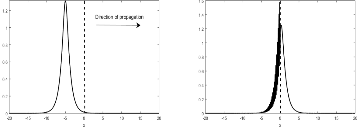
FIGURE 4. Initial profile and solution profile when interacting with the defect for Z = 10 at t = 0.174 .
