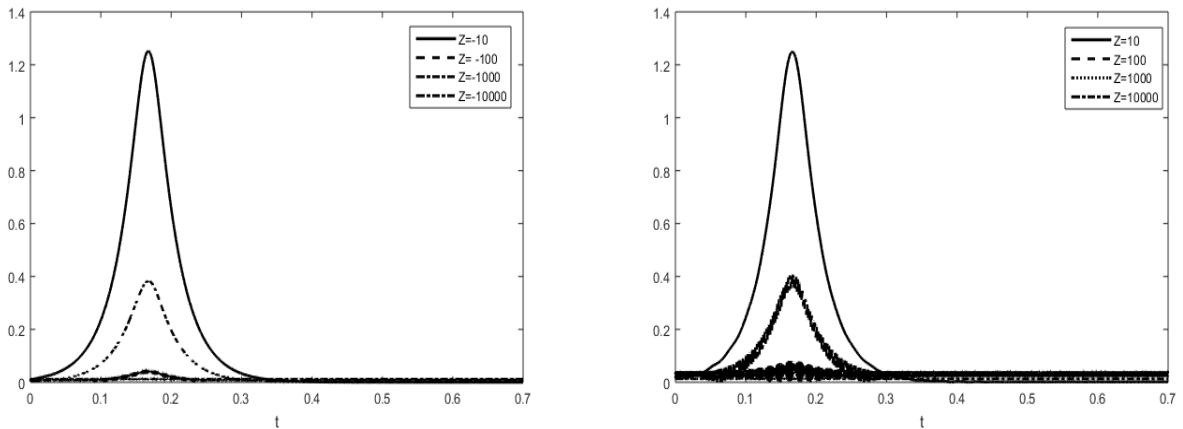
FIGURE 7. Evolution of |u(t, 0)| versus time for Z < 0 (left) and Z > 0 (right).
