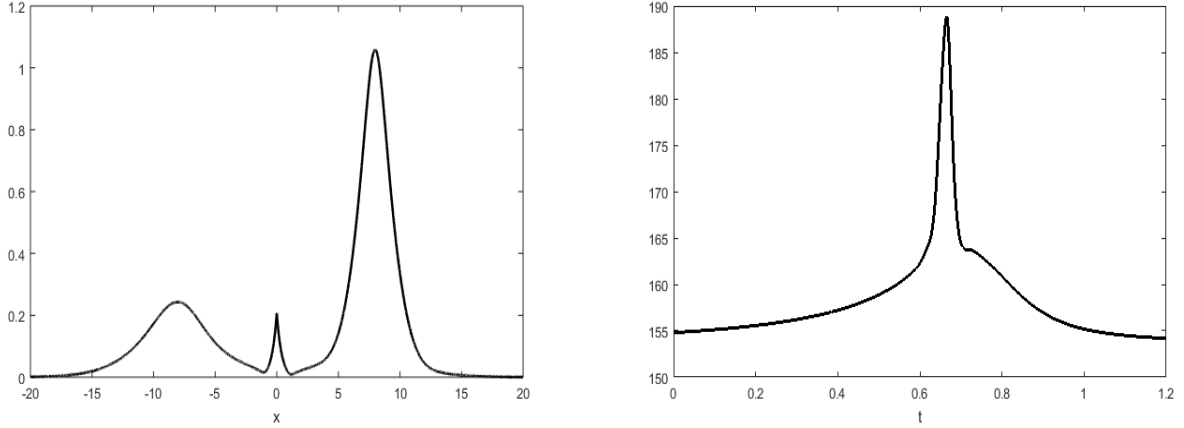
FIGURE 9. Numerical solution after the defect interaction, Z = 5 (left) and evolution of \|u_x\|_{L^2}^2 versus time for Z = 5 (right).
