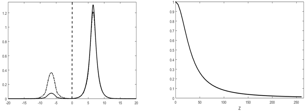
FIGURE 5. Left: Solution profile after defect interaction for two values of Z (continuous line: Z = 2 , dot-dashed line : Z = 10 ) at t = 0.3846 . Right: plot of the transmitted mass ratio \frac{M_Z^\infty}{\|u_0\|_{L^2}^2} as a function of Z .
