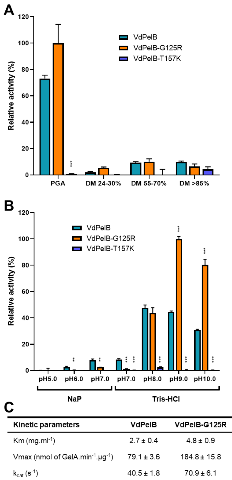
460 Fig. 4. Biochemical characterization of VdPelB
