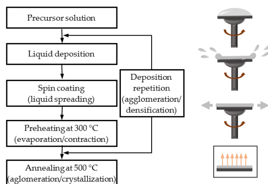
Figure 1. Deposition principle of sol-gel spin-coated ZnO samples and illustration of the liquid spreading and film formation steps.
