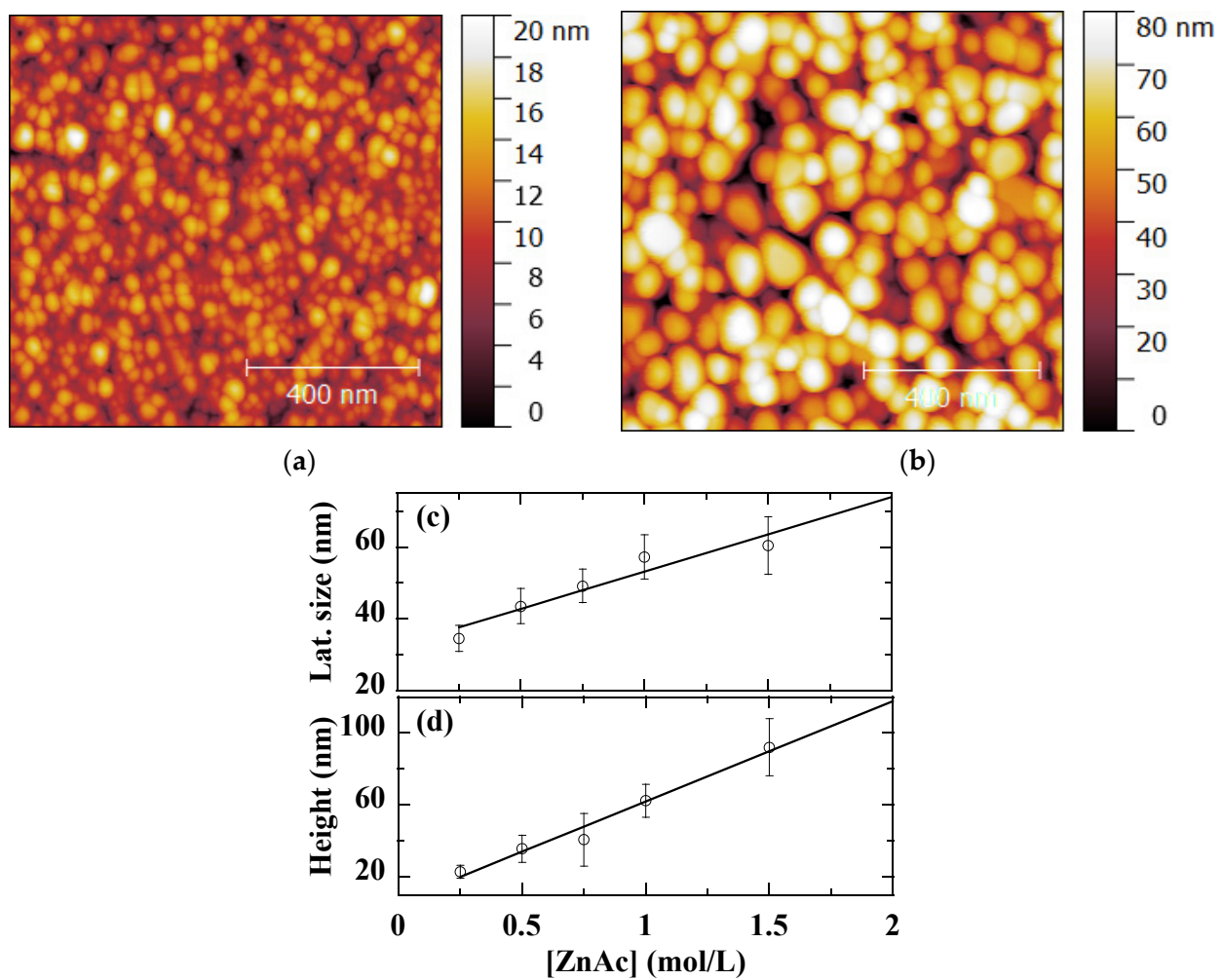
Figure 4. 1 \mu\text{m} \times 1 \mu\text{m} AFM micrographs of sol-gel spin-coated ZnO samples obtained with [\text{ZnAc}] = 0.25 \text{ mol/L} (a) and 1.0 \text{ mol/L} (b). AFM lateral size (c) and height (d) of sol-gel spin-coated ZnO samples obtained with various [\text{ZnAc}] . The straight lines are provided as guides for the eye.
