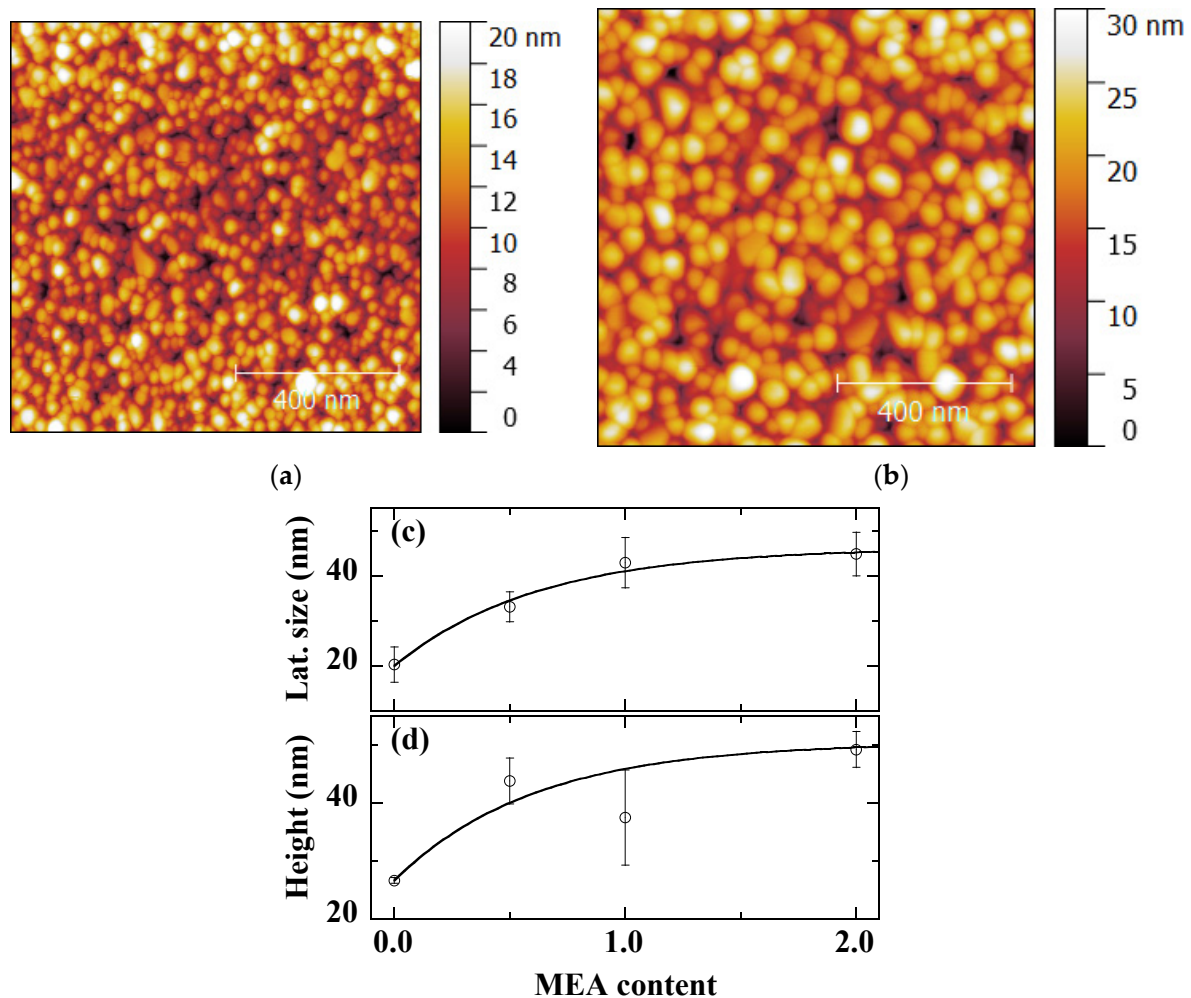
Figure 8. 1\ \mu\text{m} \times 1\ \mu\text{m} AFM micrographs of sol-gel spin-coated ZnO samples obtained with MEA contents r = 0 (a) and r = 1.0 (standard conditions) (b). AFM lateral size (c) and height (d) of sol-gel spin-coated ZnO samples obtained with various MEA contents. The curves are provided as guides for the eye.
