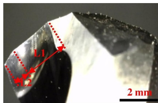
Figure 15. Definition of the principal and secondary lip lengths of the double cone drill [94].
