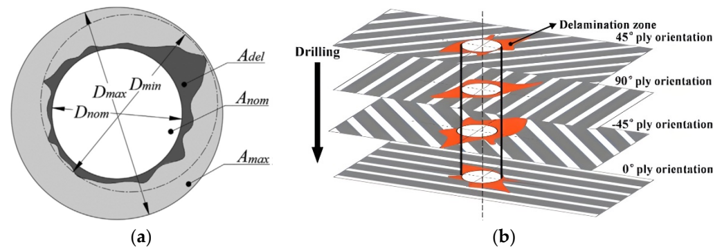
Figure 2. Drilling-induced hole damage of CFRP: (a) dimensional characteristics (diameters and areas) used to determine 1D and 2D delamination factors; (b) interlaminar delamination [71].
