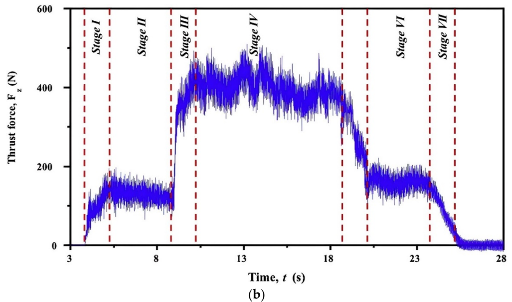
Figure 8. Drilling of CFRP/Al/CFRP co-cured materials: (a) stage division of the drilling process and (b) thrust force evolution as a function of cutting time [110].
