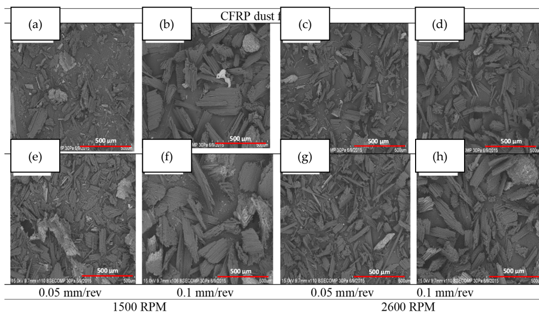
Figure 11. Dust characteristics of CFRP depending on tool geometry parameters and cutting parameters: (a–d) Point angle of 110^\circ , (e–h) Point angle of 130^\circ [95].
