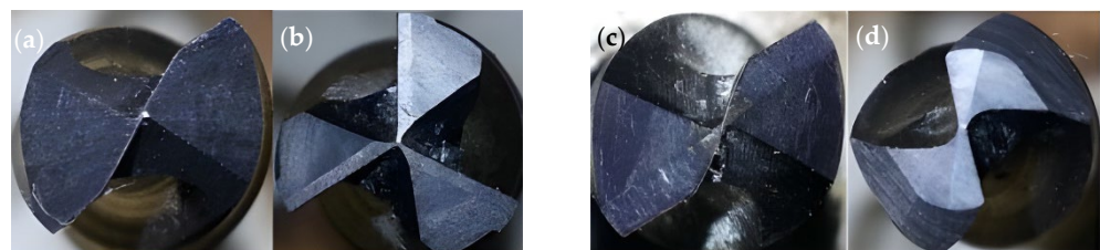
Figure 16. Drill point geometry: (a) 2-fluted, (b) 3-fluted, (c) 4-faceted and (d) 8-faceted [169].
