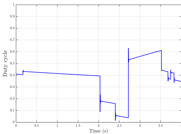
Fig. 16 – Experimental Duty-cycle for super-capacitor
