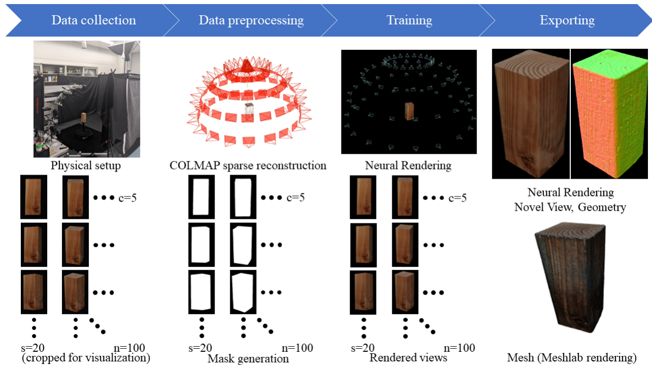
Fig. 1. Overview of our neural scanning framework. Data collection column shows our physical setup and an example of data collected of the YCB log. Data preprocessing column shows the result of intrinsic and extrinsic camera calibration using the YCB log and the result of running our mask generation tool. Training column shows the Neural Rendering of the combination of masks, original photos, camera alignment and shows the rendered views from the perspective of the training cameras. Exporting column shows a novel view of the neural scan, visualization of the surface normals (geometry), and a textured mesh exported through the neural scanning process.
