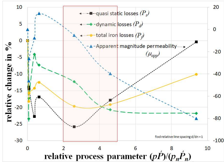
Fig. 4 : Magnetic results @1.5T@50Hz v.s. p\dot{P} .
