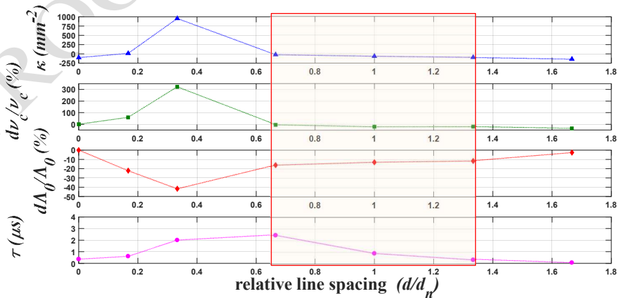
Fig. 10 : Variation of properties \kappa , v_c , \Lambda_0 and \tau v.s. line spacing d .
