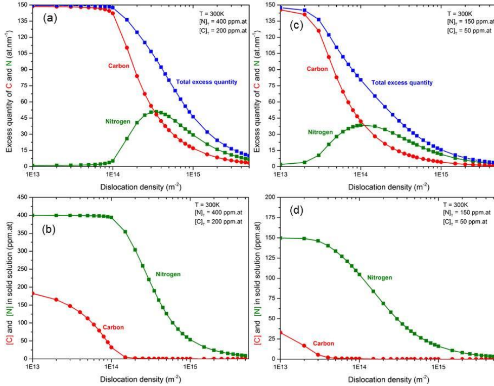
Figure 2: (a) Calculated carbon and nitrogen excess quantity (at.nm -1 ) on dislocations as a function of dislocation density (m -2 ). (b) Carbon and nitrogen remaining in solid solution as a function of dislocation density. For (a) and (b) the free concentration of carbon and nitrogen is 200 ppm.at and 400 ppm.at, respectively. (c) Calculated carbon and nitrogen excess quantity on dislocations as a function of dislocation density. (d) Carbon and nitrogen remaining in solid solution. For (c) and (d), the free concentration of carbon and nitrogen is 50 ppm.at and 150 ppm.at
