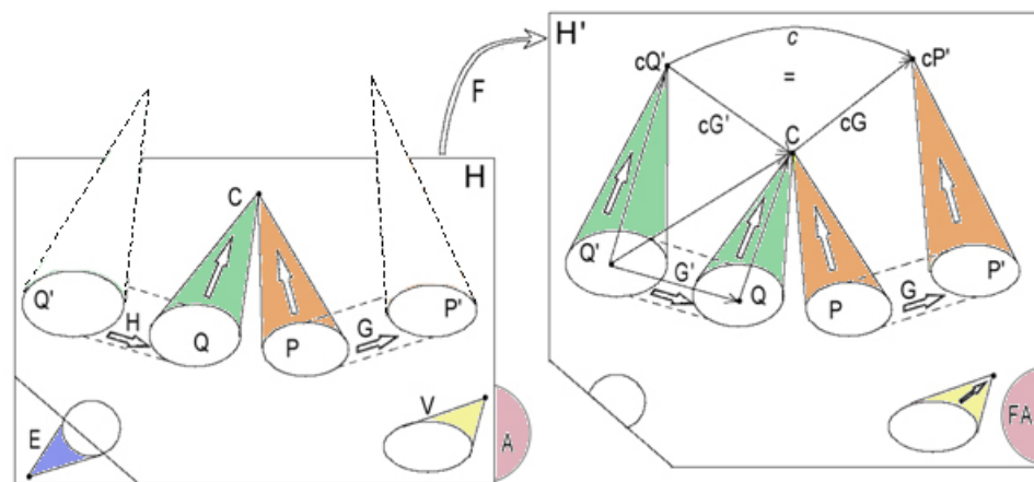
Figure 4. De/complexification process. We consider the procedure Pr on H with objectives: to add the set A, to suppress the cone E, and to add colimits cP' and cQ' to the diagrams P' and Q'. The de/complexification H' 'optimally' adds the colimit cones of bases Q' and P' , the simple links cG and cG' binding the clusters G and G' and the complex link c: cQ' \rightarrow cP' which is their composite.
