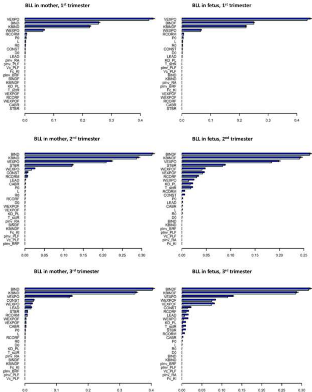
Figure S 2: FOI (light blue) and TOI (blue) from the Sobol sensitivity analysis: Pb Levels in the fetus blood and mother blood at the 1 st , 2 nd and 3 rd trimesters of pregnancy.
