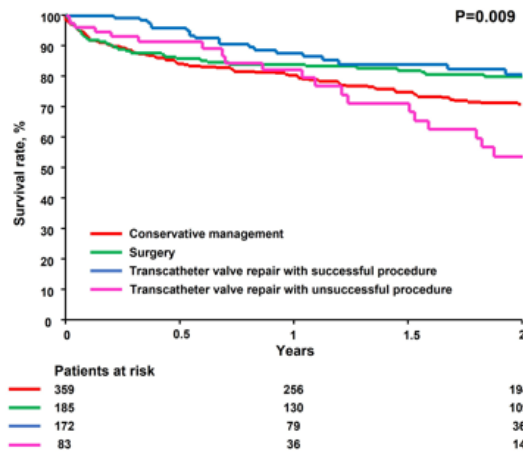
INTERMEDIATE TRI-SCORE (4-5)
