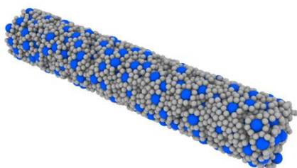
Figure 5. Microstructures and properties of the obtained electrodes for a highly cohesive (case D) and low cohesive (case C) pastes.
