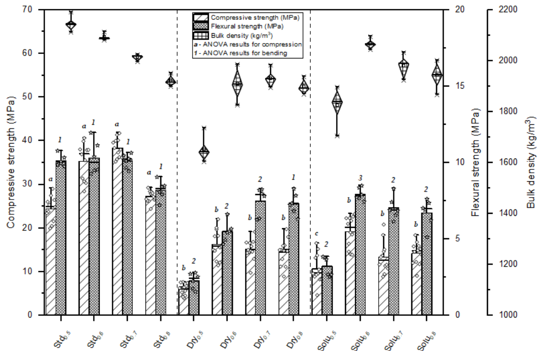
Figure 5 • Flexural and compressive strengths plotted with bulk densities of 90 days admixed mortars with the W/C ratio influence. Different numbers and letters above the bar charts indicate a significant difference ( p < 0.05 ) from other formulation with the same W/C ratio.
