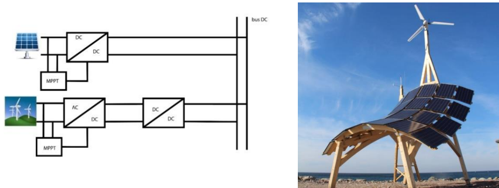
Figure 1. Diagram of a photovoltaic-wind hybrid system
