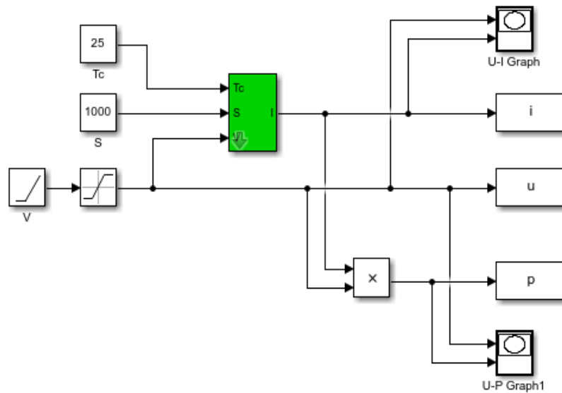
Figure 4. PV simulation diagram of PV
