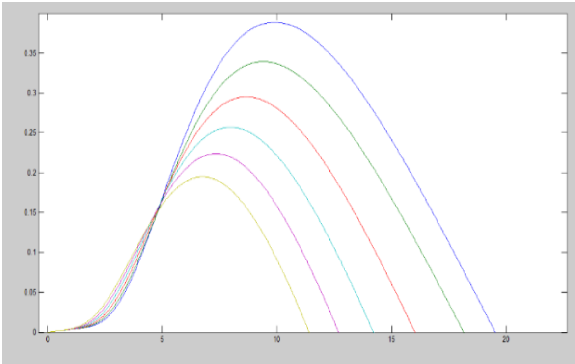
Figure 8. Curve of variation of Cp from lamda
