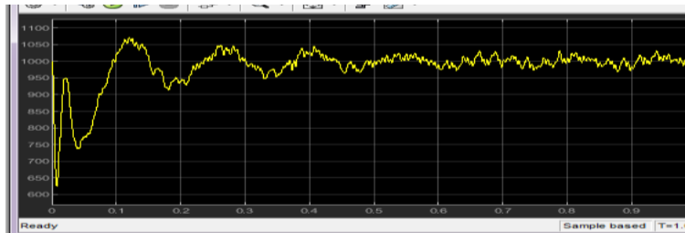
Figure 14. Courbe of tension Bus DC HVDC
