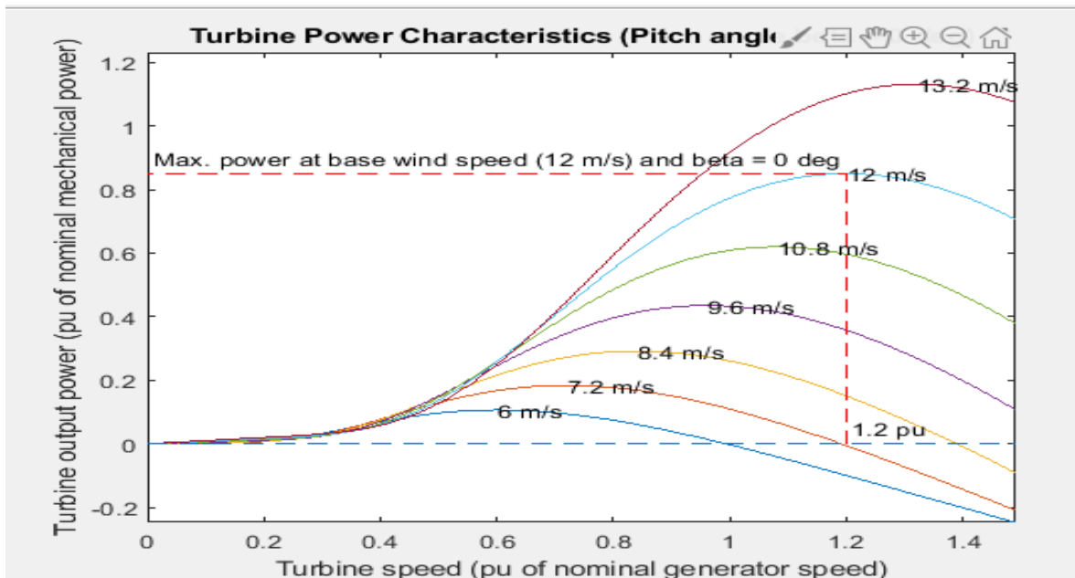
Figure 7. Power variation curves from speed.
