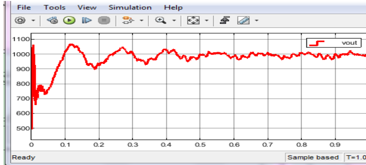
Figure 12. Courbe of tension Bus DC of PV
