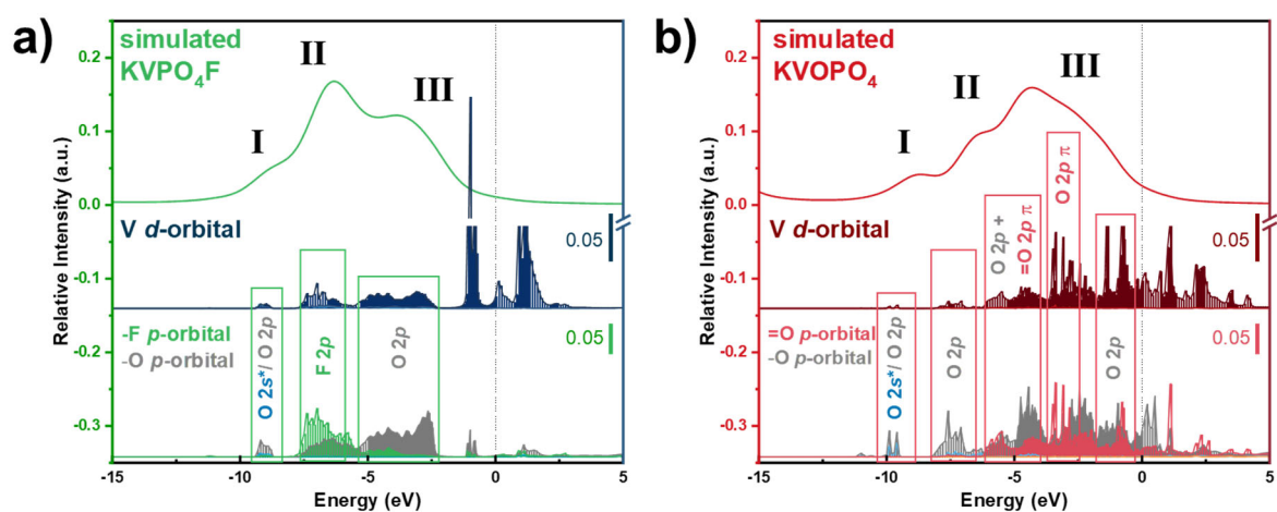
Figure 6. a-b) Simulated VtC K \beta XES of KVPO 4 F and KVOPO 4 and with their corresponding densities of states (DOS) at the K \beta 2,5 region, and c) the experimental spectra (open circles) along with the peak deconvolution (solid lines)
