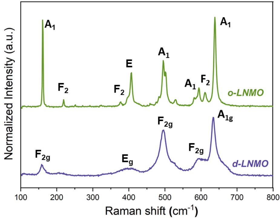
Figure 2: Raman spectra of prepared LNMO samples. The intensity was normalized based on the peak observed at \sim 500\text{ cm}^{-1} , sensitive to the Ni oxidation state and its coordination (here unchanged, as there is only \text{Ni}^{2+} ).
