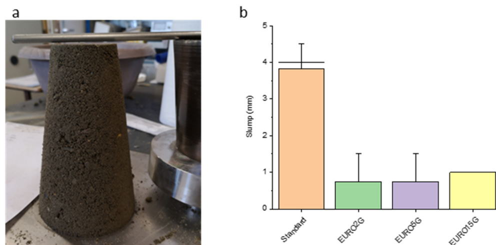
Figure 3. Slump test (a) of the mortars and the results (b).
