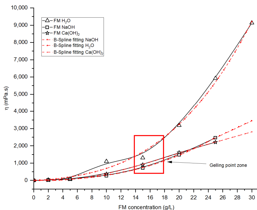
Figure 1. Apparent viscosity of FM solutions at 20 \pm 2 °C (60 rpm).
