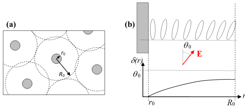
Figure 12: (a) The polymer fibres are modelled as cylinders of radius r_0 separated by 2R_0 . (b) Boundary conditions of the angle \delta .
