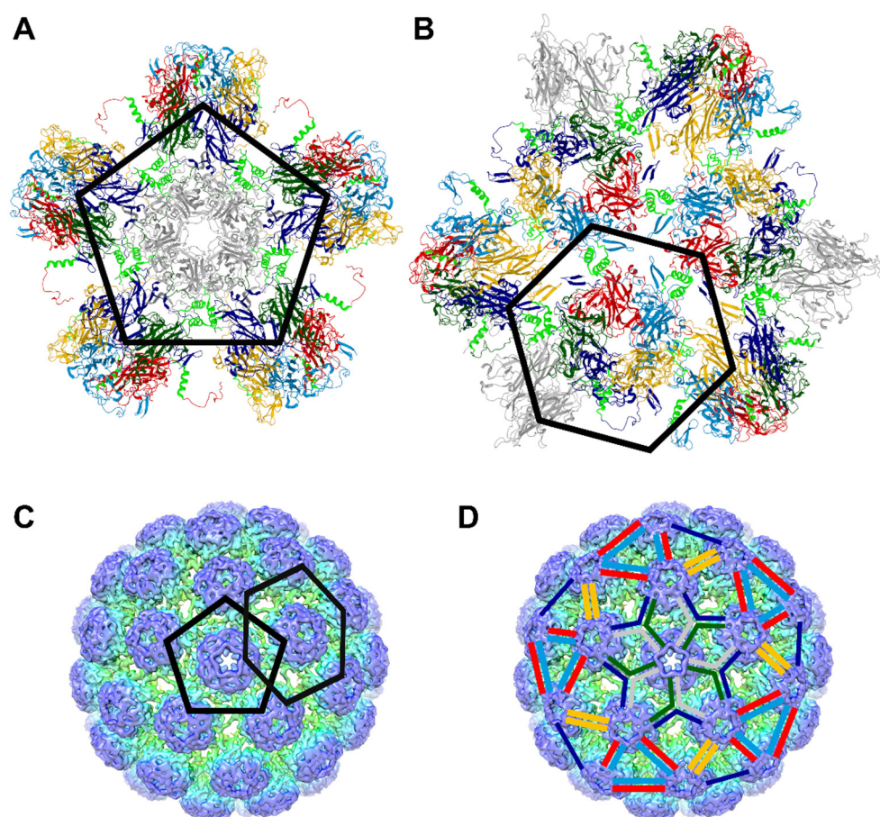
Figure 4. Location of the Y300, P301 and L305 amino acids in the structure of BKPyV viral capsid. (A,B) VP1 monomers of pentavalent pentamers are shown in gray whereas VP1 monomers of hexavalent pentamers are shown in red, green, blue, cyan and yellow. The amino acids 297 to 314 of each VP1 monomer, encompassing the “pentapeptide hinge” (297–301) and the C helix (302–314) are highlighted in light green. Images were created using Mol* Viewer [42] and obtained from the Research Collaboratory for Structural Bioinformatics Protein Data Bank (rcsb.org) [43] (PDB ID: 6ESB [6]). (C) The respective positions of pentavalent and hexavalent pentamers on the viral capsid structure are highlighted at the center of a pentamer and a hexamer, respectively. (D) The C-terminal arms of VP1 monomers are highlighted using the color code used in panels A and B. Panels C and D have been produced from https://pdj.org/emnavi/data/emdb/media/3283/images/emd_3283.tif (accessed on 19 February 2022) [7,44].
