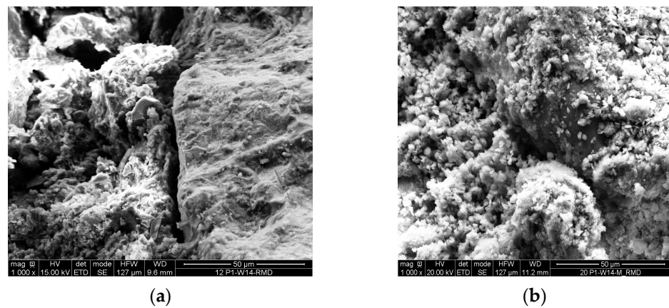
Figure 13. Interfacial transition zone in the case of composites elaborated with (a) 12% of matrix and non-matured bottom ash or (b) 20% of matrix and matured bottom ash.
