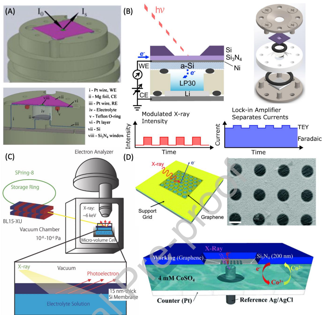
Figure 2.2.2. Enclosed electrochemical cells for XPS and XAS of battery interfaces. a) XAS cell sealed with \sim 100 nm \text{SiN}_x membrane, used primarily for FY measurements [60]; b) TEY-XAS cell and lock-in approach for separating faradaic and TEY currents, used to study SEI formation on a-Si [63]; c) Silicon membrane approach for studying solid-liquid interfaces with XPS using \sim 6 keV X-ray excitation [64]; d) Graphene Membrane approach for studying the solid-liquid interfaces with XPS, so far demonstrated with aqueous electrolytes [65,66].
