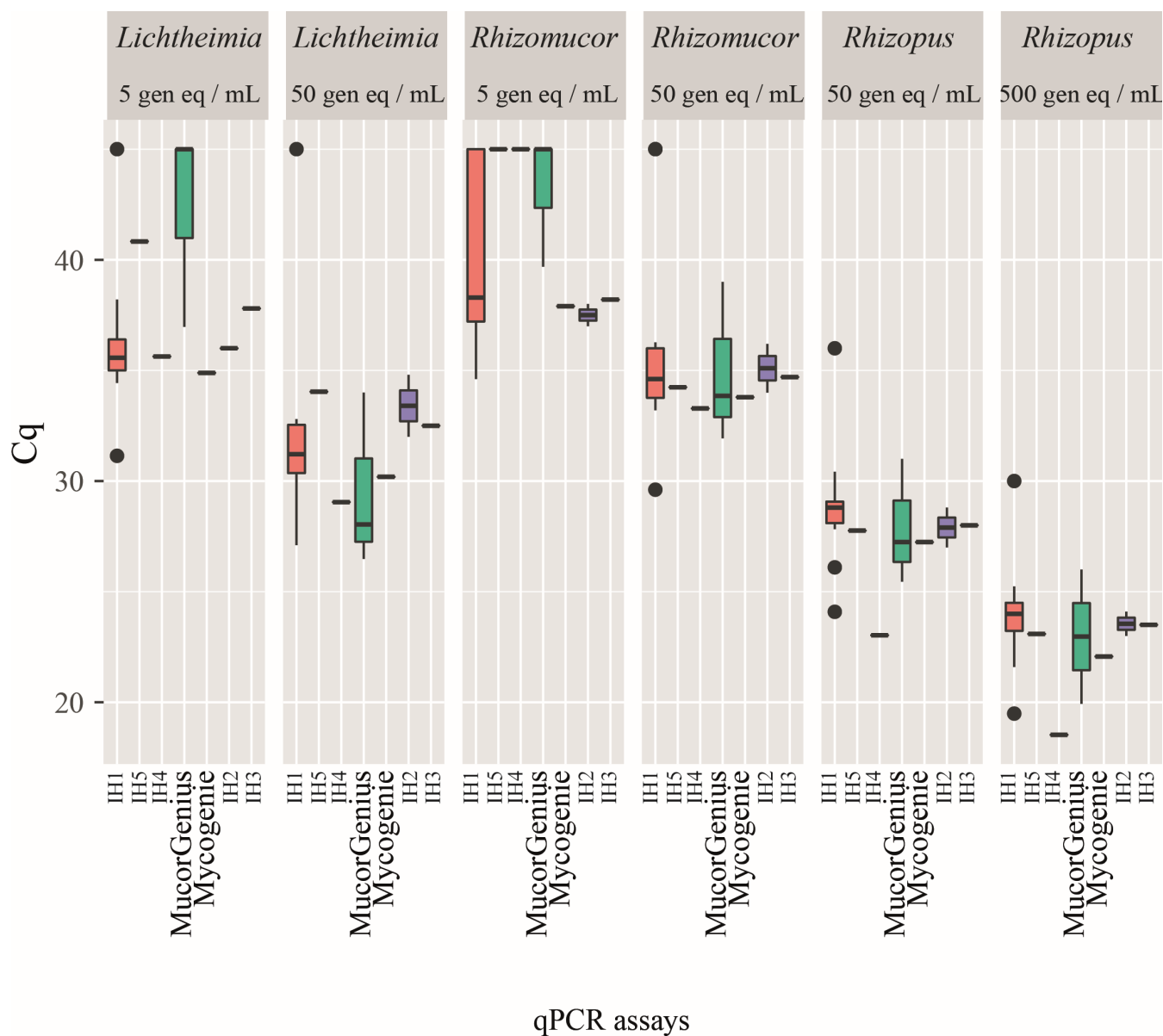
FIG 3 Distribution of Cq values according to qPCR assays ( n = 22 centers, 132 qPCR trials [four centers excluded from the analysis due to lower positivity rates]). IH: in-house qPCR assays described in papers as follows: IH1: ref. (2), IH2: ref. (18), IH3: ref. (6), IH4: ref. (19), IH5: ref. (20). Negative results were allocated a value of 45 cycles.
