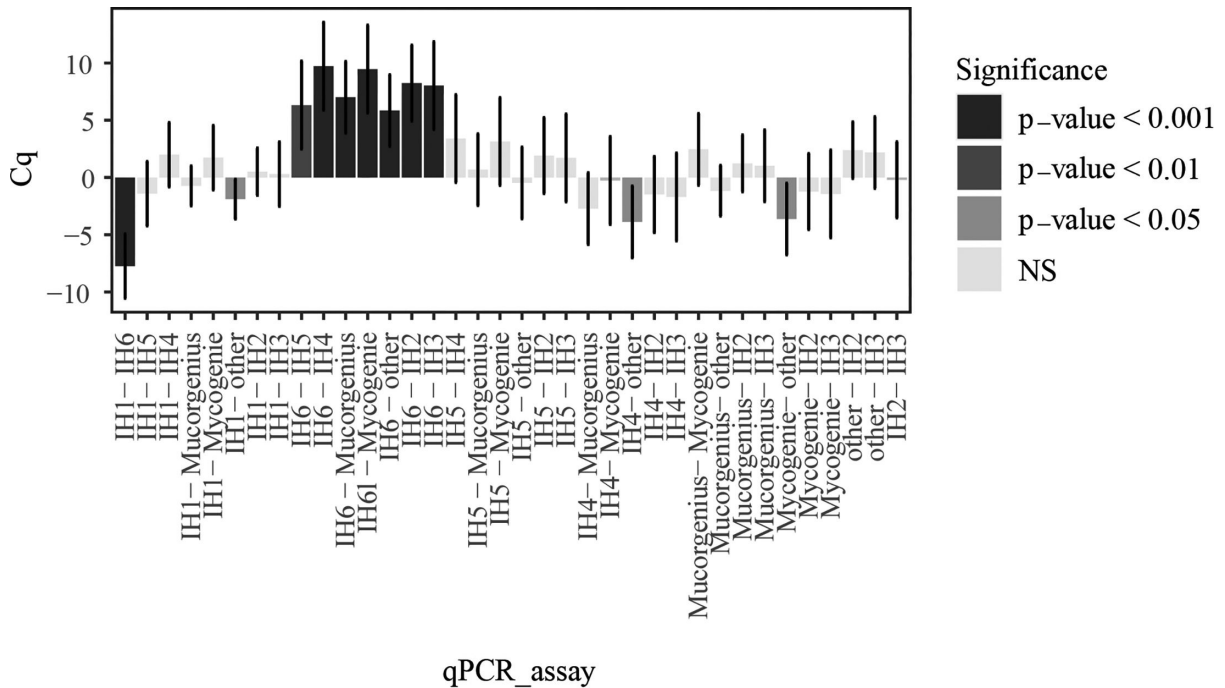
FIG 2 Pairwise comparison of the quantification cycle (Cq) values generated by the qPCR assays (least squares means and confidence intervals between the qPCR assay included in the fixed part of linear mixed effects model). Significance of differences is mentioned with gray intensities. When the difference had a negative value, the first qPCR assay had a best performance and vice versa. NS: no significant difference. Negative results were allocated a value of 45 cycles. IH: in-house qPCR assays described in papers as follows: IH1: ref. (2), IH2: ref. (18), IH3: ref. (6), IH4: ref. (19), IH5: ref. (20), IH6: ref. (21). Other: in-house unpublished method.
