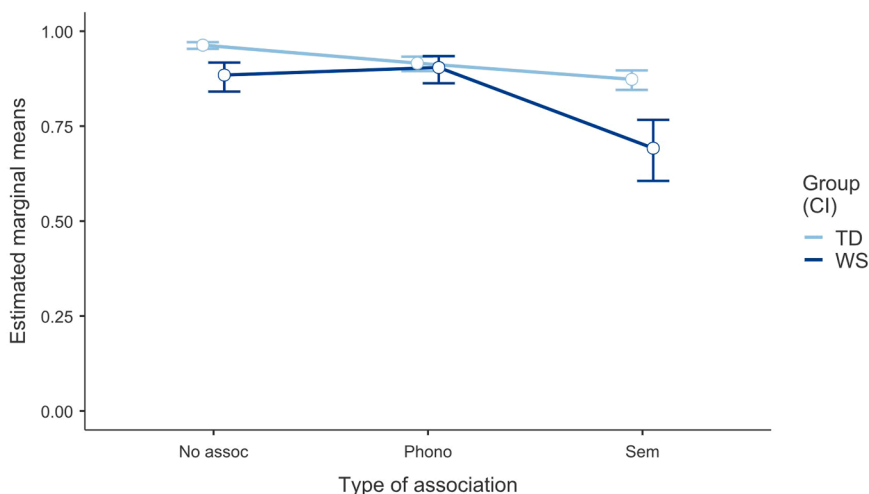
Fig. 2. Estimated marginal means of answer accuracy by association type and group for the GLMM with EVIP as a covariate. Note. 95 % CIs are presented.
